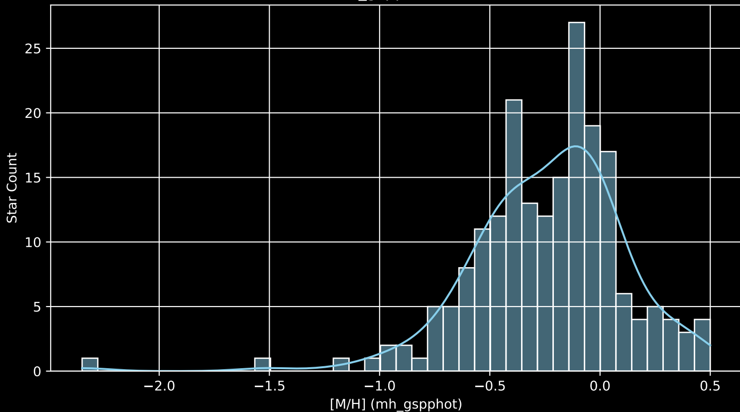
APOGEE DR17 Field: [217+49_MGA [M/H] (mh_gspphot) (n= 200)
