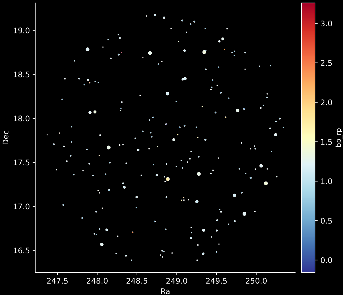
APOGEE DR17 Field: [217+49_MGA] Stars: 201
